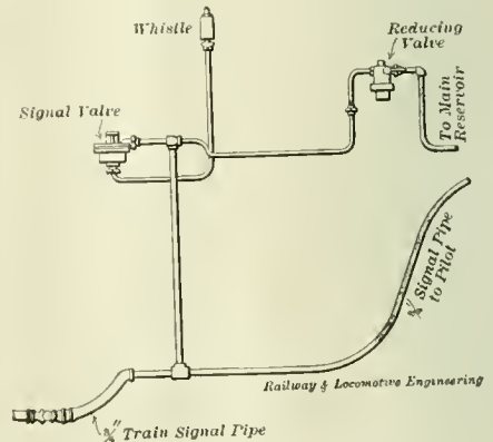
FIG. 4.—SIGNAL PIPING.
